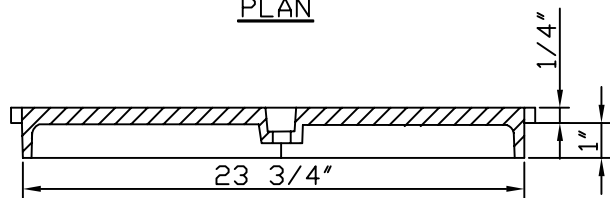
SEC 'A-A'
